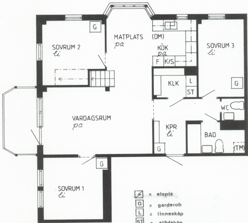
UNDRE PLAN
